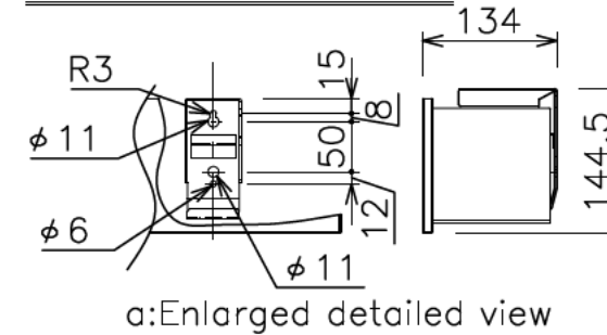
Sliding Bracket(S=1/8)
