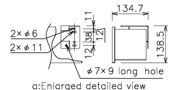
Side Bracket(S=1/8)
