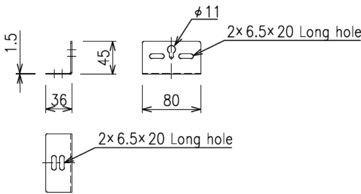
Detail of screen bracket S=1:5
