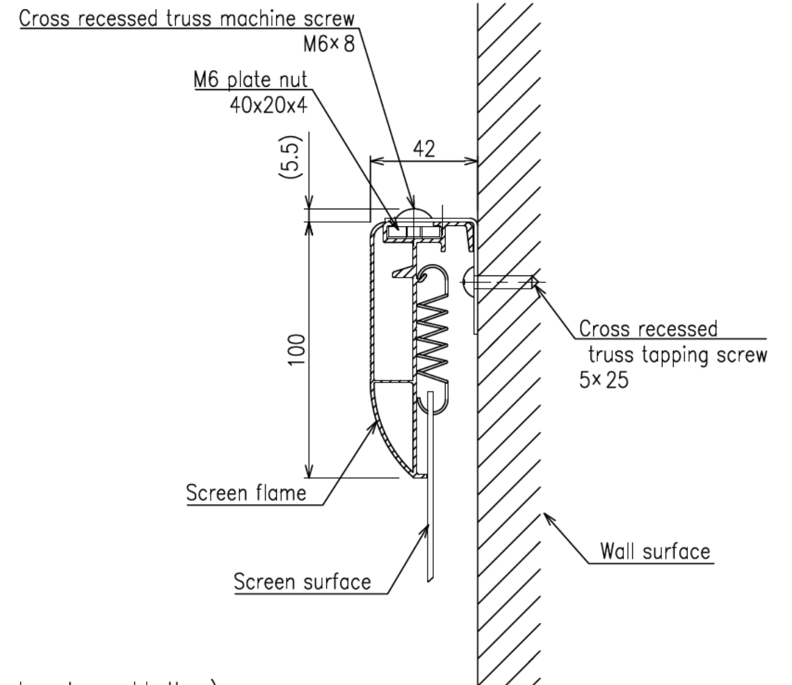
Screen bracket (2 places each on top and bottom)
