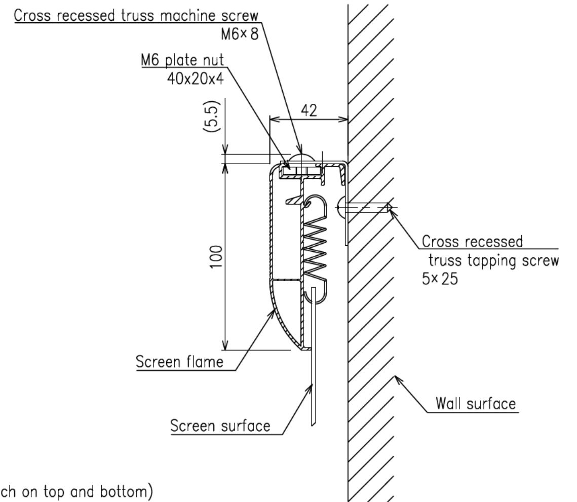
Cross-section A-A
