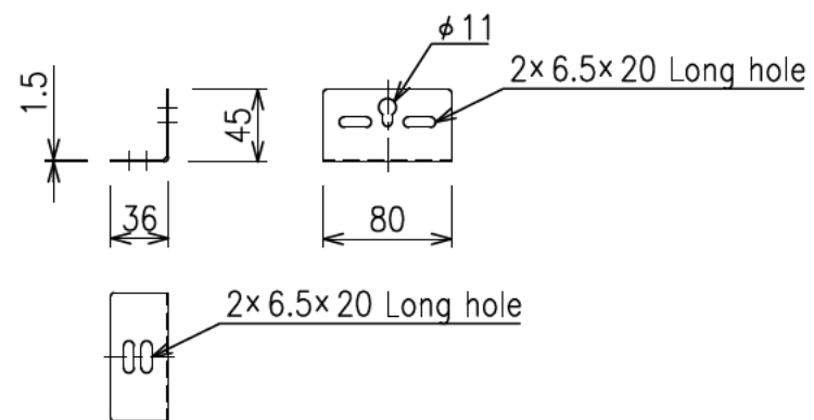
Detail of screen bracket S=1:5
