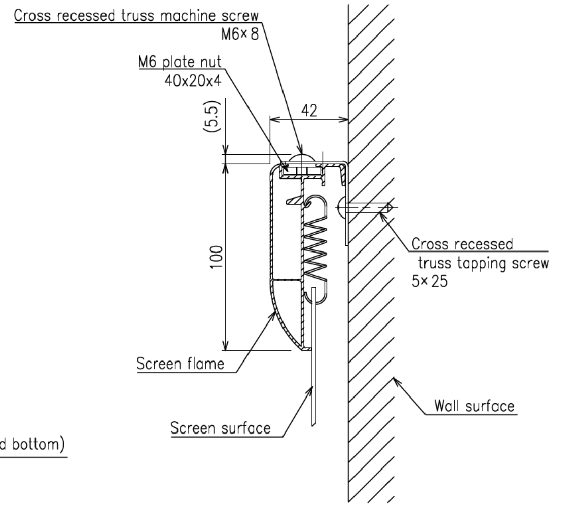
Cross-section A-A
