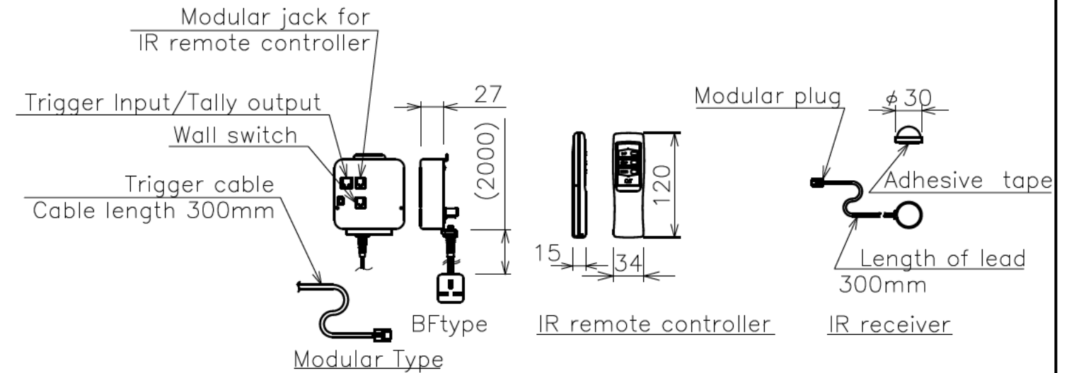
Circuit box and control switch(S=1/6)
