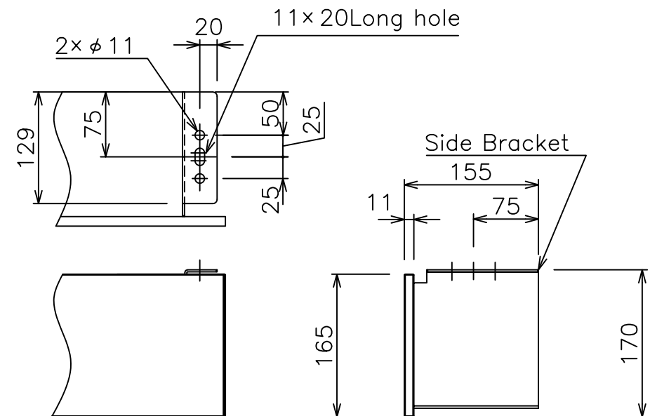
Detail of Side bracket (S=1/6)
