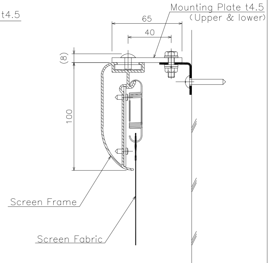
Section A-A 1/2
