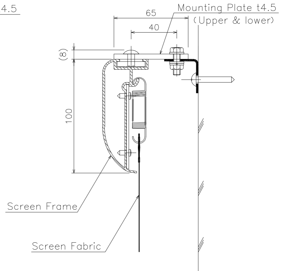
Section A-A 1/2
